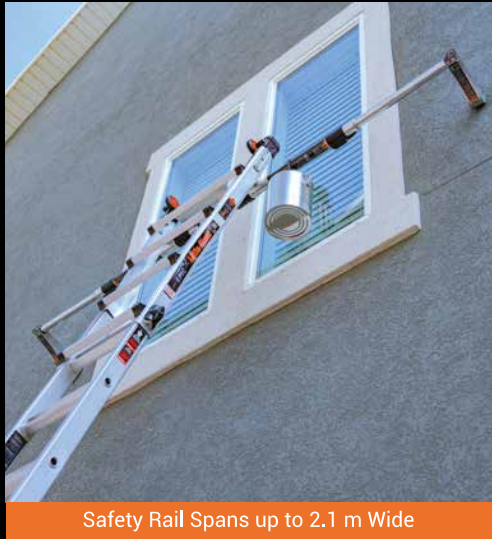
Safety Rail Stand-Off Position
